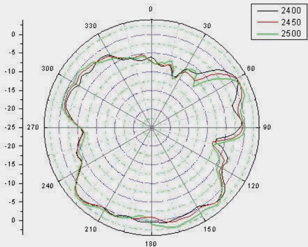
2.4G (PHI=0)
